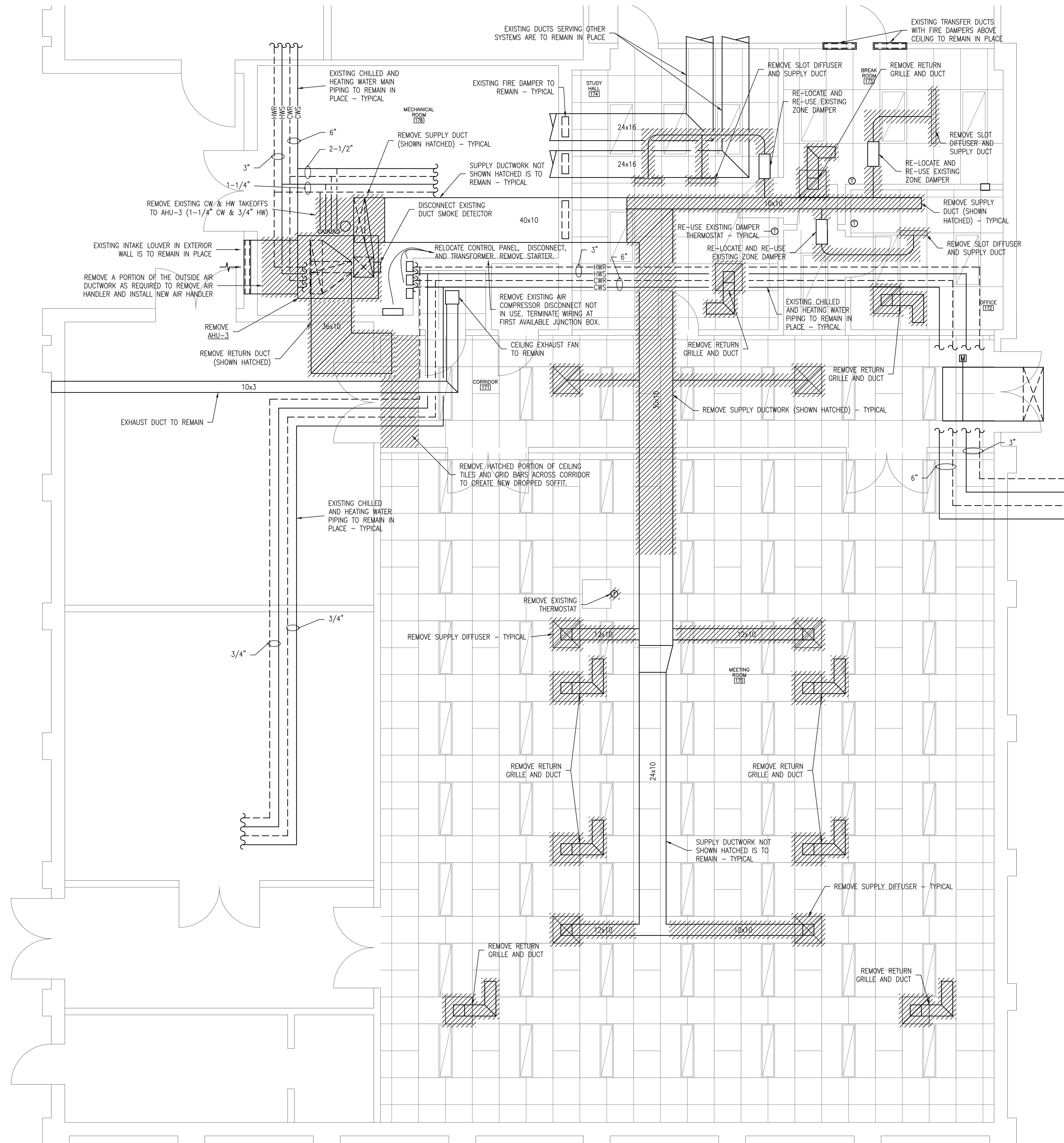
HVAC DEMOLITION FLOOR PLAN SCALE: 1/4" = 1'-0"
