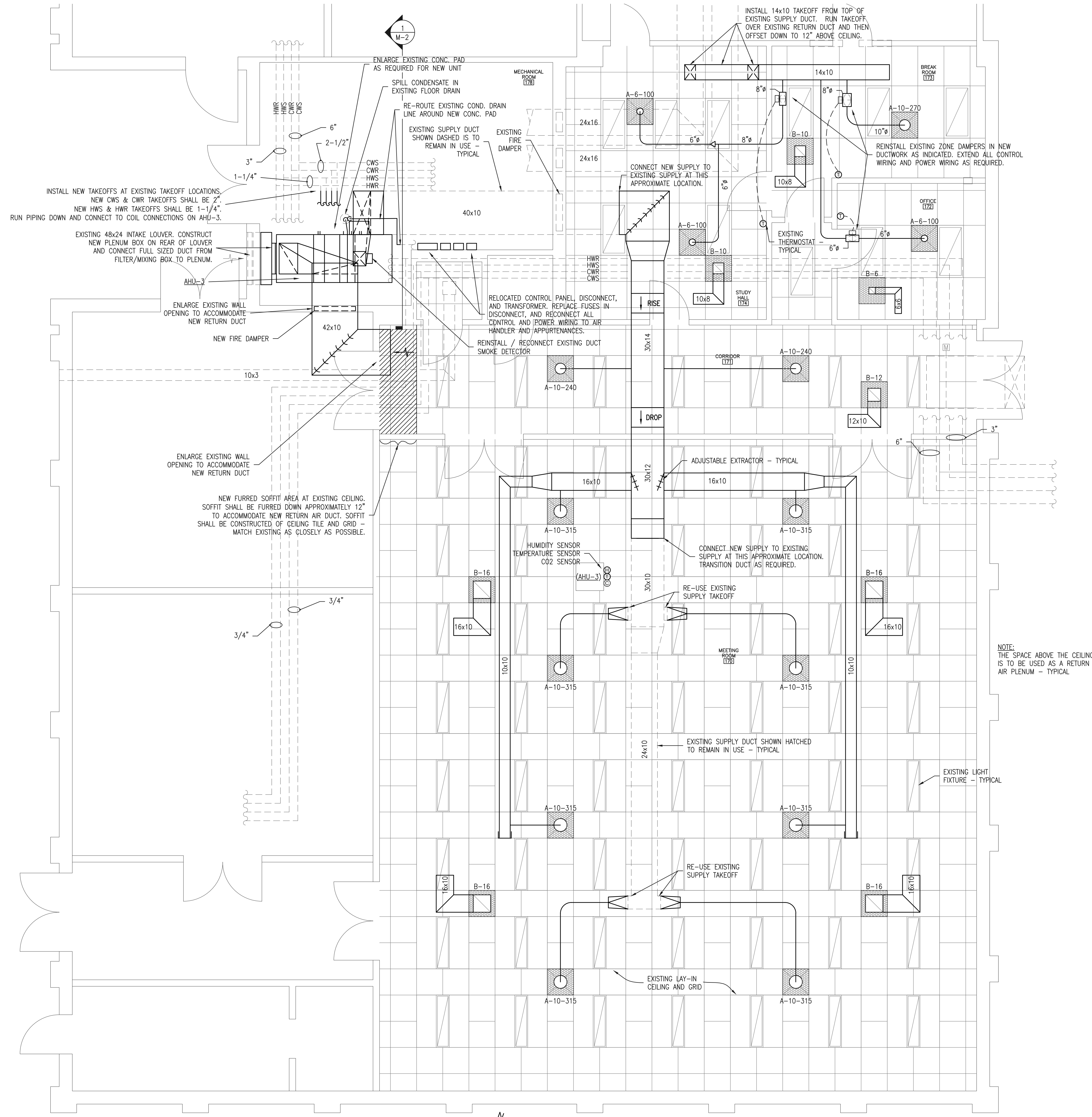
HVAC RENOVATION FLOOR PLAN SCALE: 1/4" = 1'-0"
